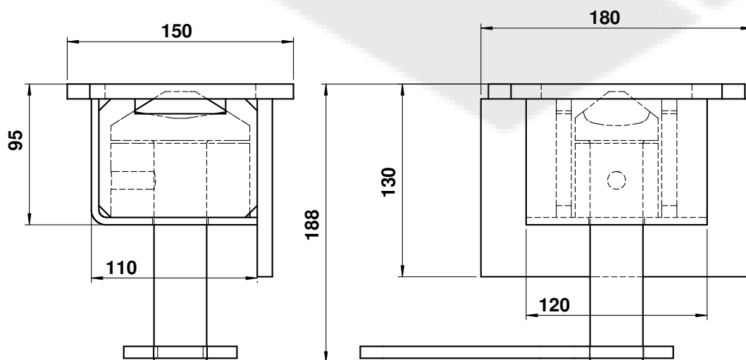
TWISTLOCK IN HIDDEN POSITION
