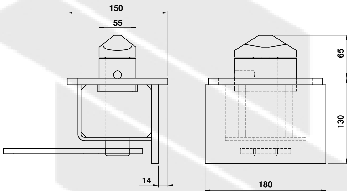
TWISTLOCK IN WORKING POSITION
