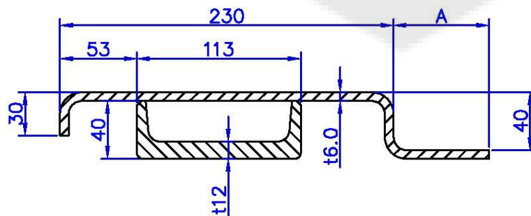
Rear Corner Post with Inner Channel
