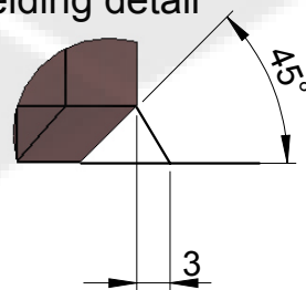
Welding detail
